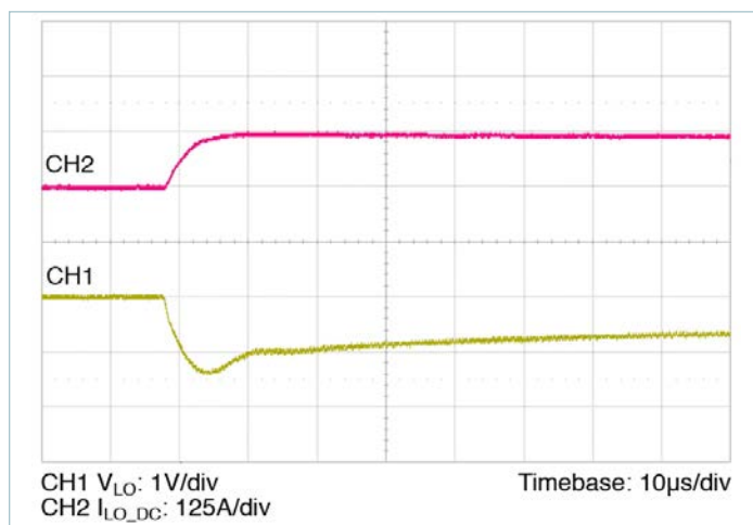
Figure 15 — 0 – 125A transient response: C_{HI\_IN\_EXT} = 10\mu F , no external C_{LO\_OUT\_EXT}
