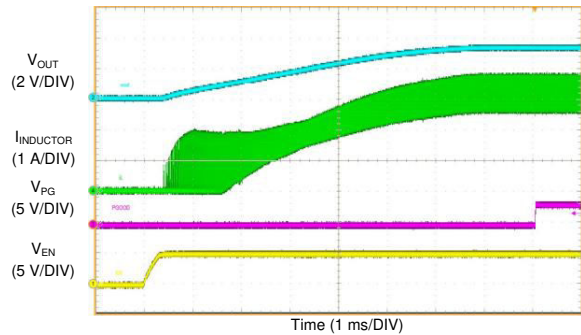
图 10-31. LM61460-Q1 Start-up with 50-mA Load
