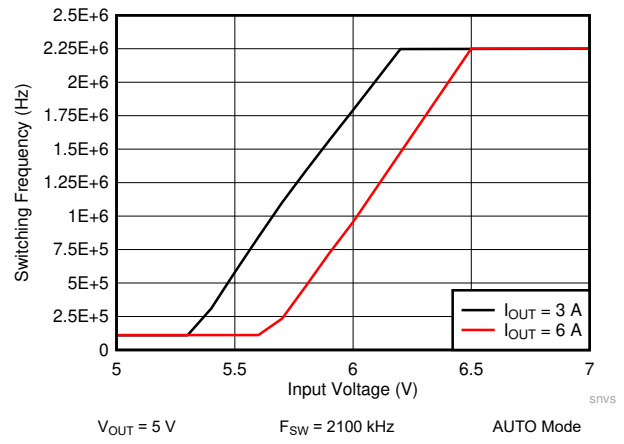
图 10-28. LM61460-Q1 Frequency Dropout Curve
