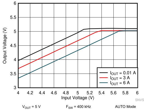
图 10-23. Dropout Curve
