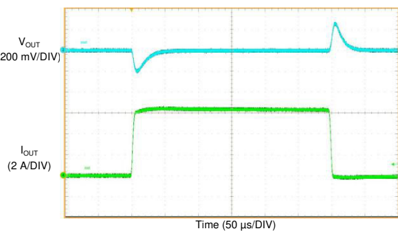
图 10-37. Graceful Recovery from Dropout
