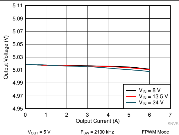
图 10-20. LM61460-Q1 Load and Line Regulation
