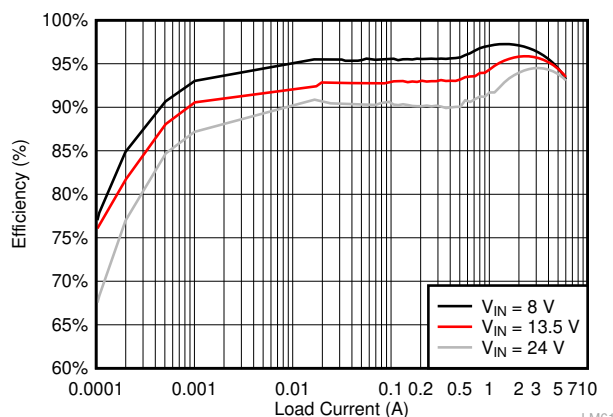
效率: V_{OUT} = 5V , f_{SW} = 400\text{kHz}
