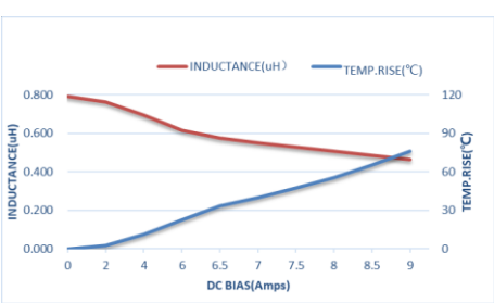
ZETC252012SR82MBT-LF
