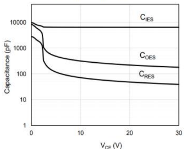
Fig.6 Typical capacitance
