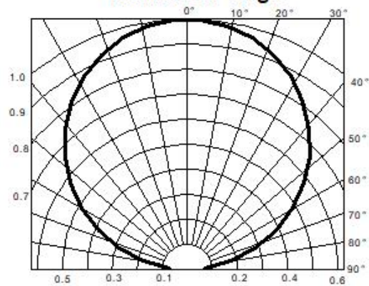
Radiation angle
