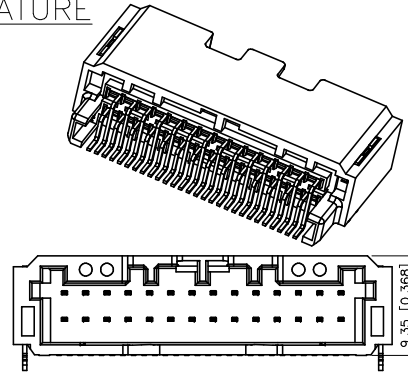
28 PIN
