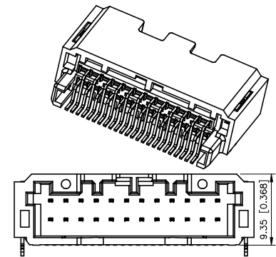
24 PIN
