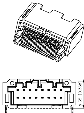
16 PIN
