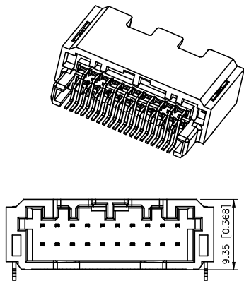
20 PIN
