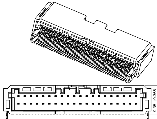
40 PIN
