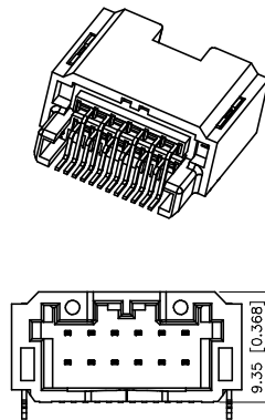
12 PIN
