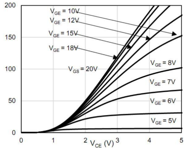
Fig.2 Output Output characteristics (150°C)
