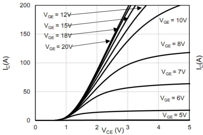
Fig.1 Output Output characteristics (25°C)
