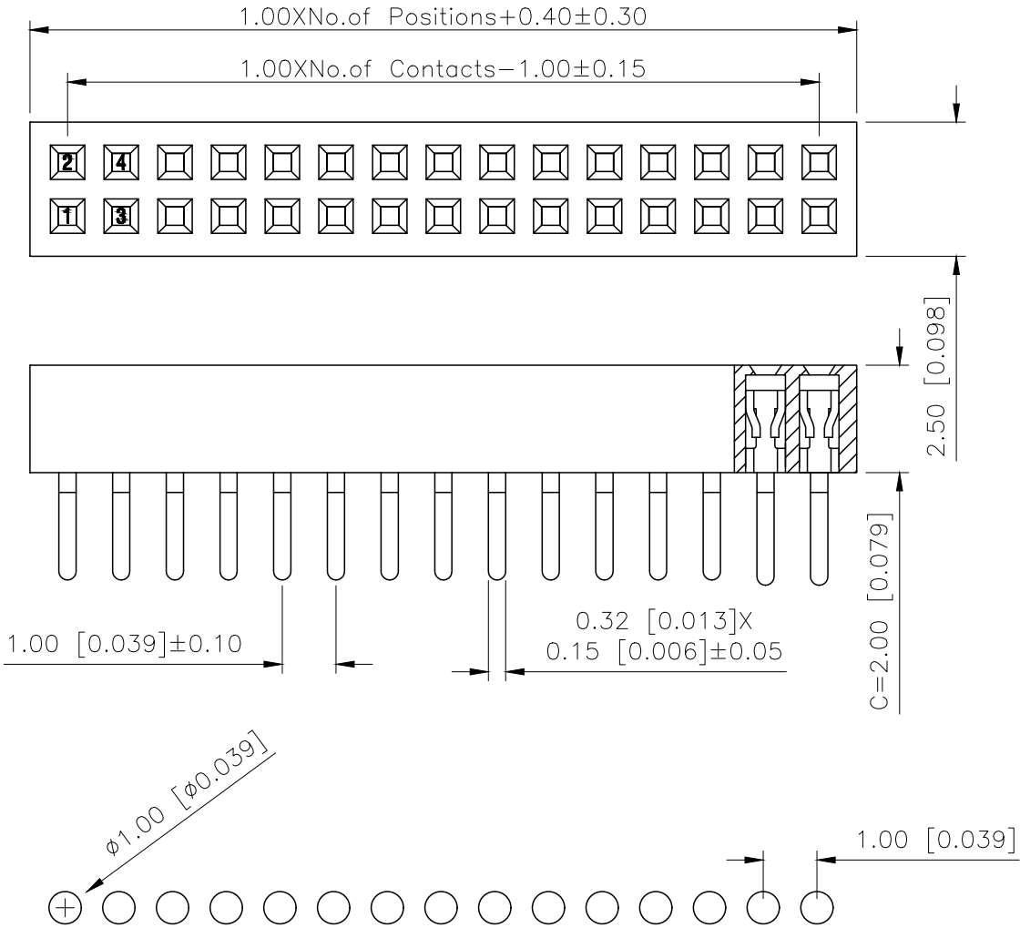
PCB LAYOUT
