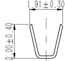
SECTION: E-E
