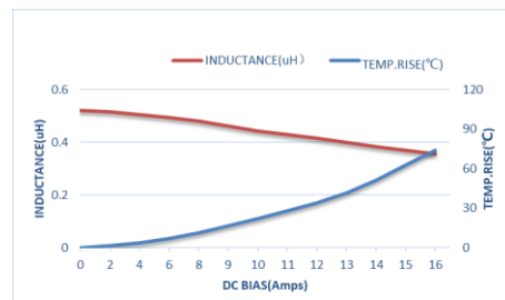
ZEMS303020-R50M
