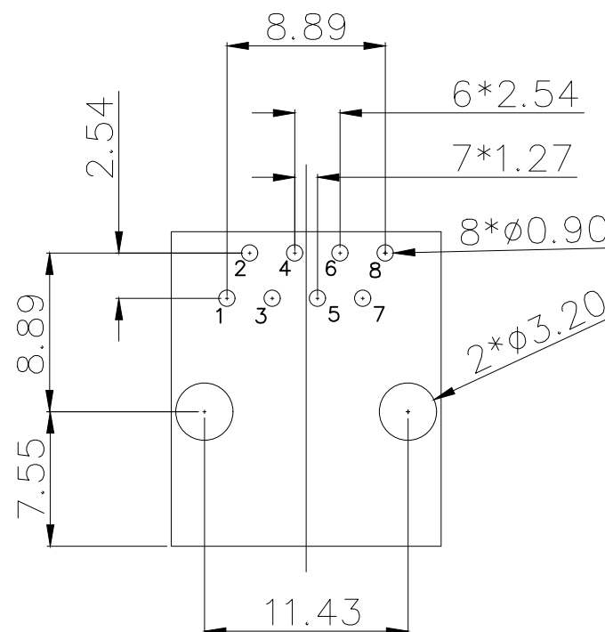
RECOMMENDED PCB LAYOUT TOP VIEW(TOL: ±0.05)
