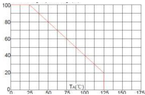
Pulse Derating Curve
