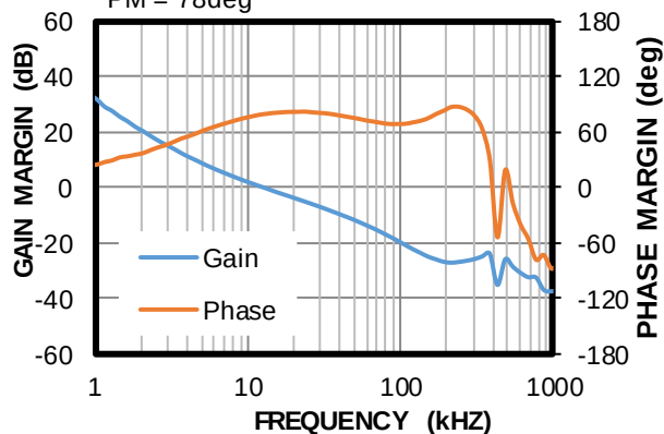
Bode Plot
