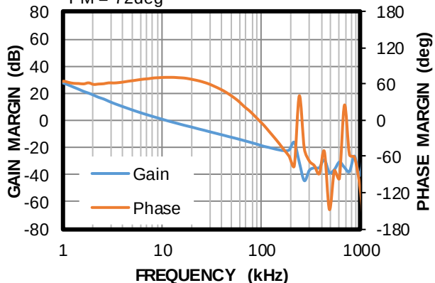
Bode Plot
