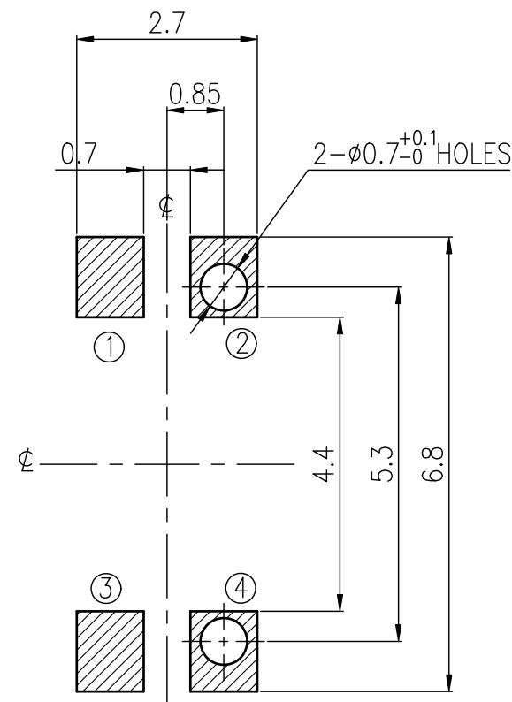
HATCHED AREA SHOWS SOLDERING LAND
