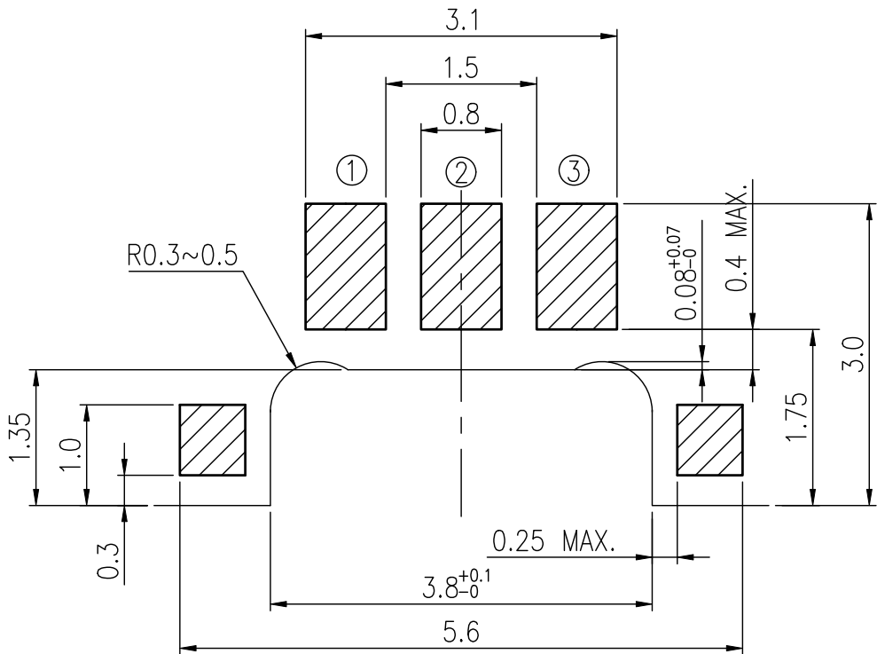
P.C.B LAYOUT (VIEW FROM THE DIRECTION A)
