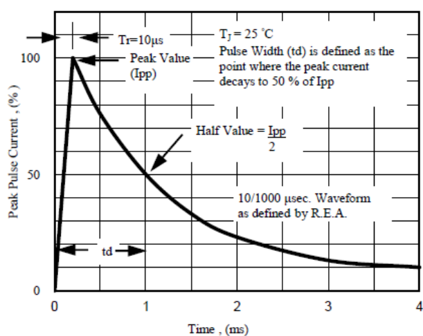
Fig. 5 - Pulse Waveform
