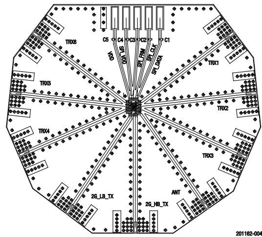
Figure 4. SKY18106-455LF Evaluation Board Assembly Drawing
