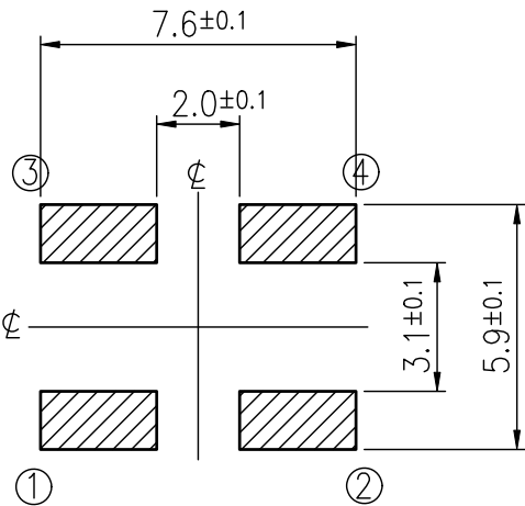
HATCHED AREA SHOWS SOLDERING LAND
