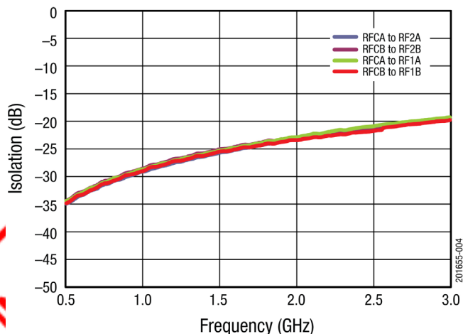
Figure 4. Isolation vs Frequency
