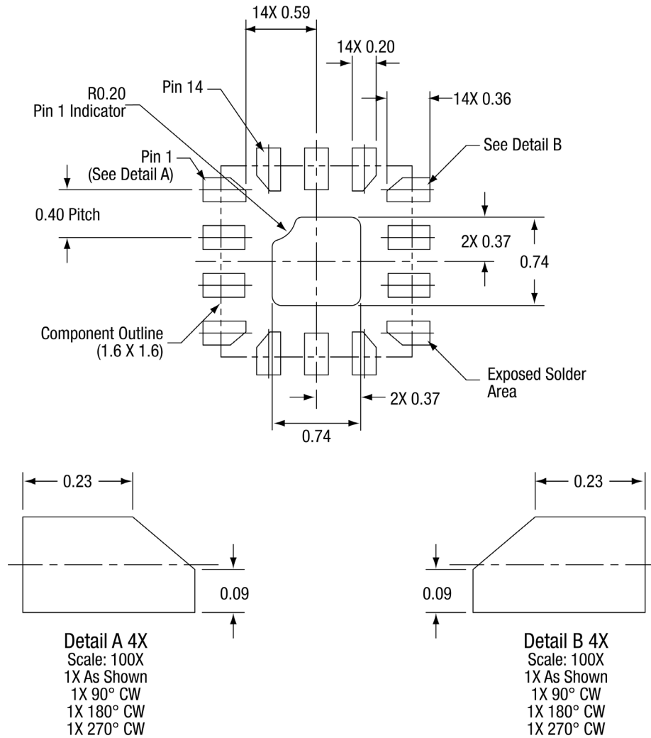
Figure 9. SKY13421-486LF PCB Layout Footprint (Top View)
