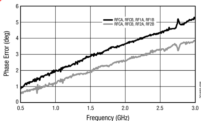
Figure 6. Phase Error vs Frequency
