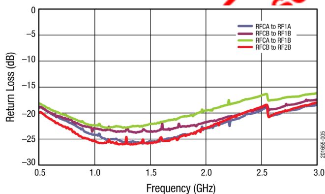
Figure 5. Return Loss vs Frequency
