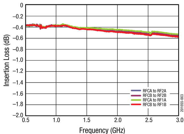
Figure 3. Insertion Loss vs Frequency
