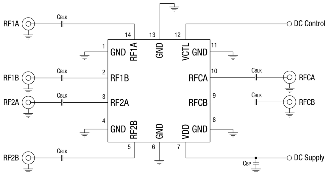
Figure 7. SKY13421-486LF Evaluation Board Schematic
