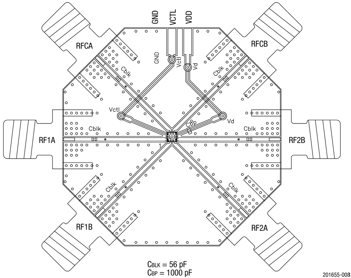
Figure 8. SKY13421-486LF Evaluation Board Assembly Diagram
