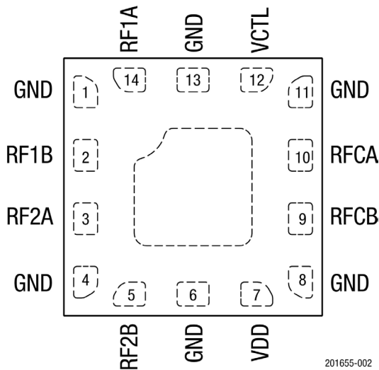
Figure 2. SKY13421-486LF Pinout (Top View)
