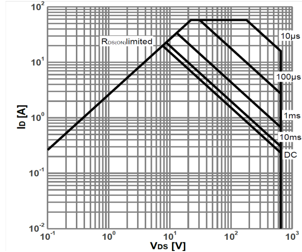
Figure 5: Safe operating area For TO-220、TO-247、TO-263
