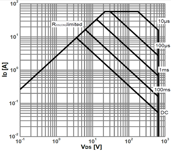
Figure 6: Safe operating area For TO-220F
