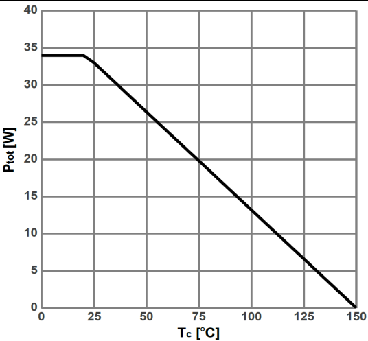
Figure 4: Power dissipation For TO-220、TO-247、TO-263
