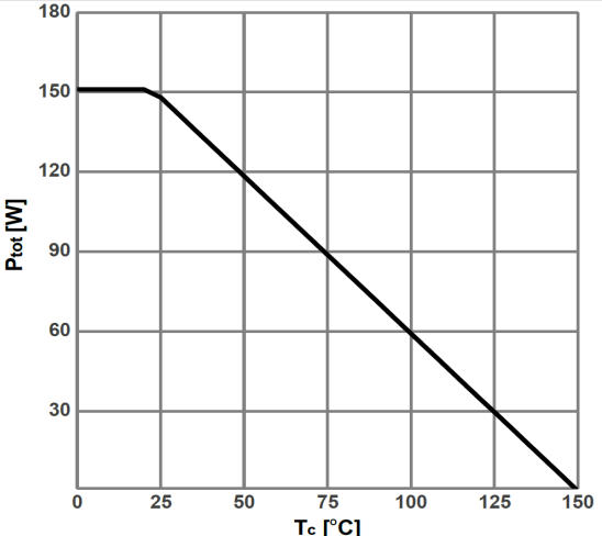
Figure 4: Power dissipation For TO-220、TO-247、TO-263
