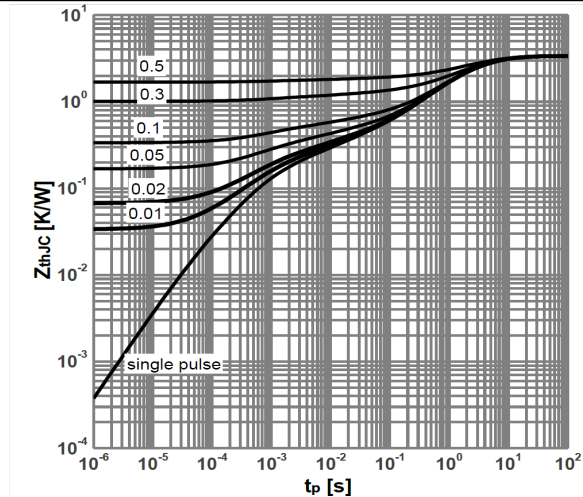
Figure 3: Transient Thermal Impedance For TO-220、TO-247、TO-263
