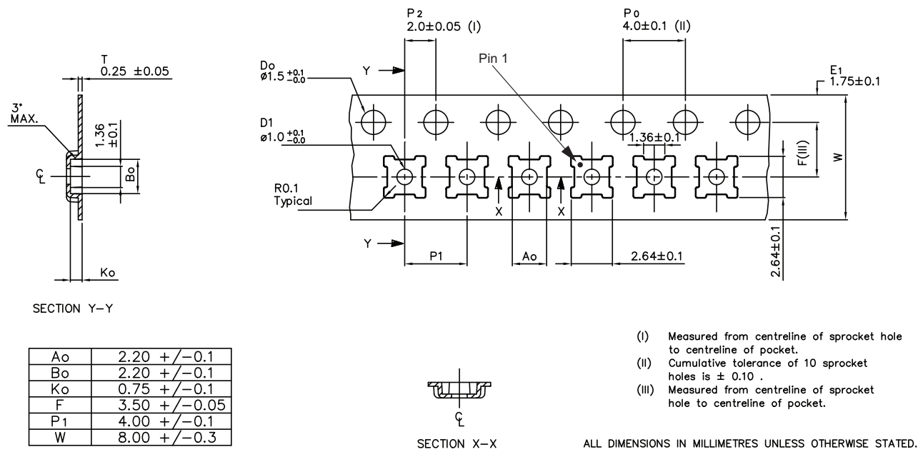
Figure 8. Tape and Reel Dimensions
