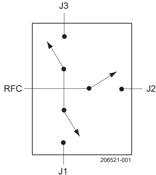
Figure 1. Block Diagram
