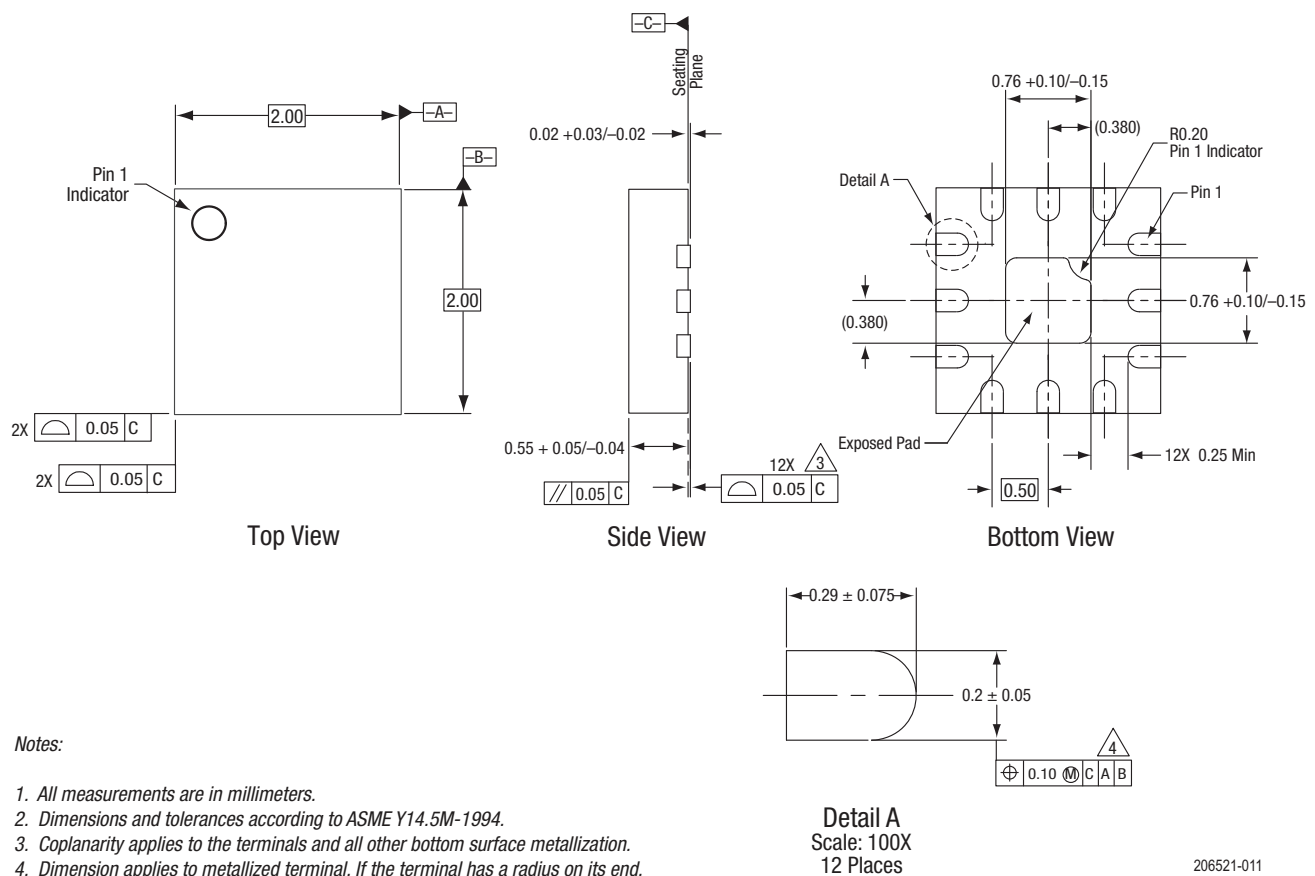
Figure 7. Package Dimensions
