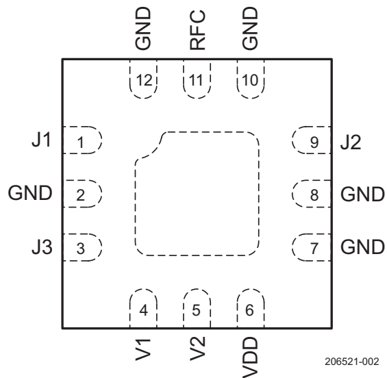
Figure 2. Pinout (Top View)
