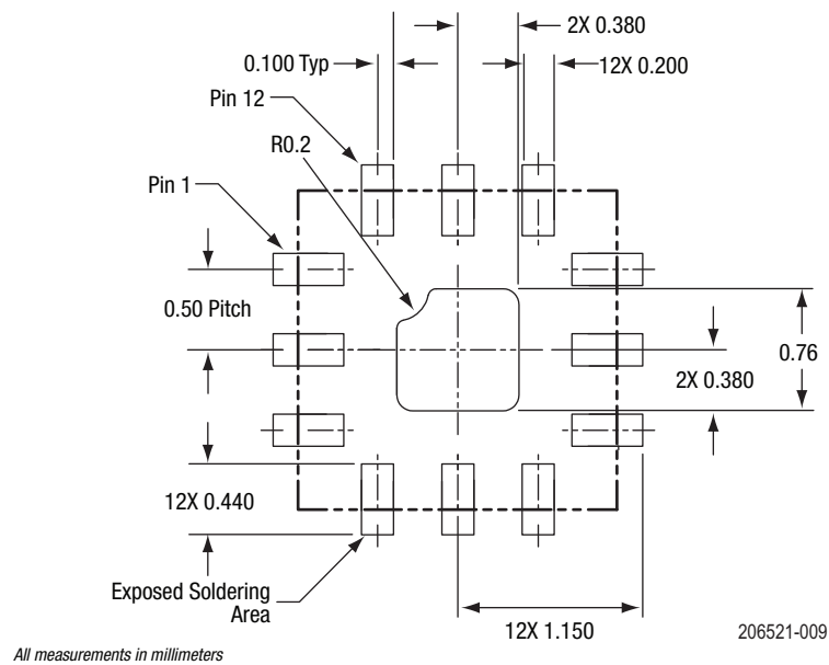
Figure 5. PCB Layout Footprint (Top View)
