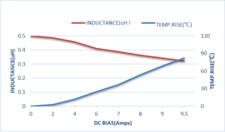
ZEPIM252012S-R47M
