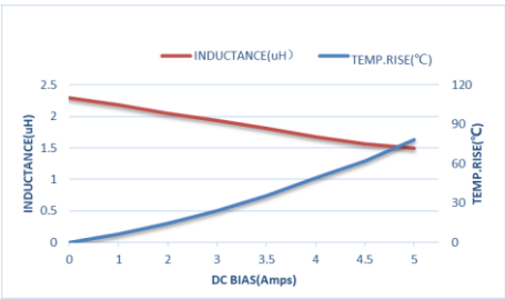
ZEPIM252012S-2R2M
