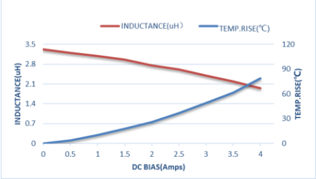
ZEPIM252012S-3R3M
