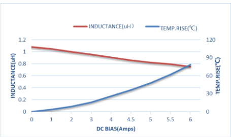
ZEPIM252012S-1R0M
