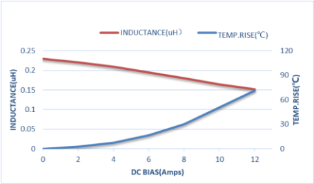
ZEPIM252012S-R22M
