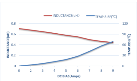
ZEPIM252012S-R68M
