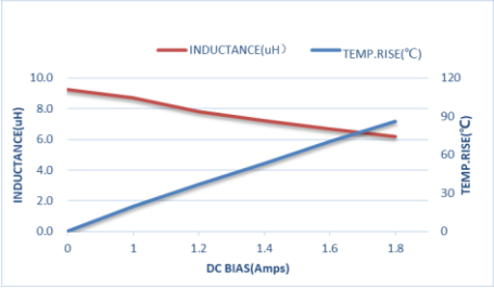
ZEPIM252012S-100M
