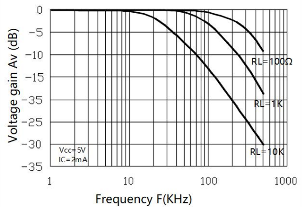
Fig.10 Frequency Response
