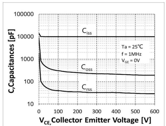
Fig.6 Typical capacitance
