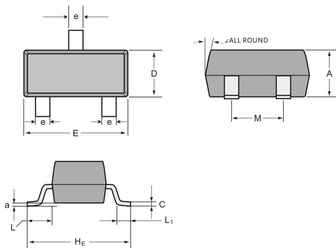
SOT-23 mechanical data
