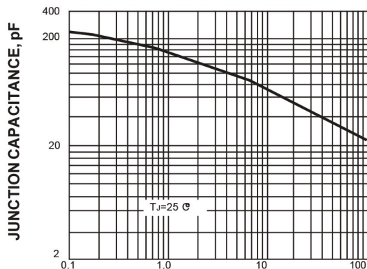
FIG. 5-TYPICAL JUNCTION CAPACITANCE
