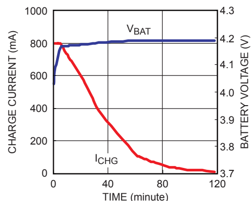
800mA Charge Curve
