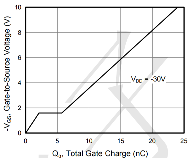
Figure 8. Gate Charge
