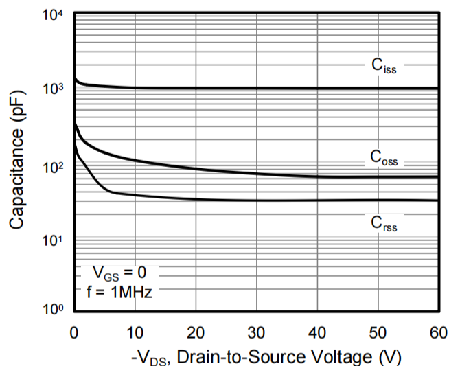
Figure 7. Capacitance
