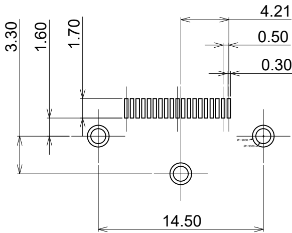
PCB LAYOUT(TOP VIEW) (T=1.60mm)
