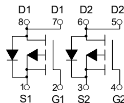
SOP-8 (SO-8)
