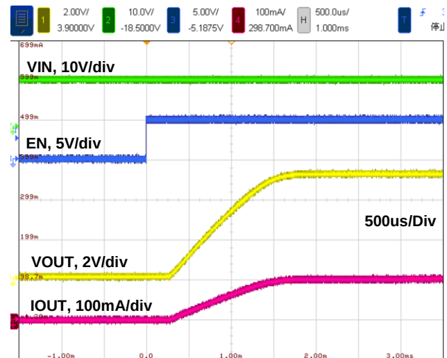
Figure 17. Startup by EN, 50Ω load
