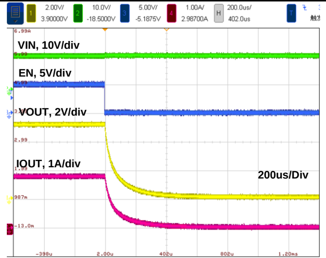
Figure 20. Shutdown by EN, 3Q load
