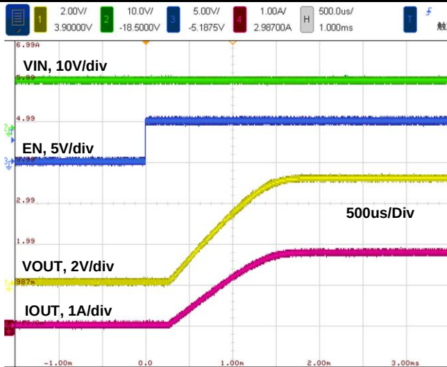
Figure 19. Startup by EN, 3Q load
