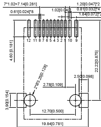
RECOMMENDED PCB LAYOUT VIEWED FROM COMPONENT SIDE
