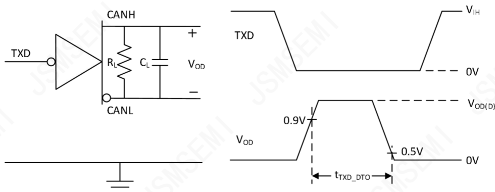
Figure5-6. TXD Dominant Timeout Test Circuit and Measurement
