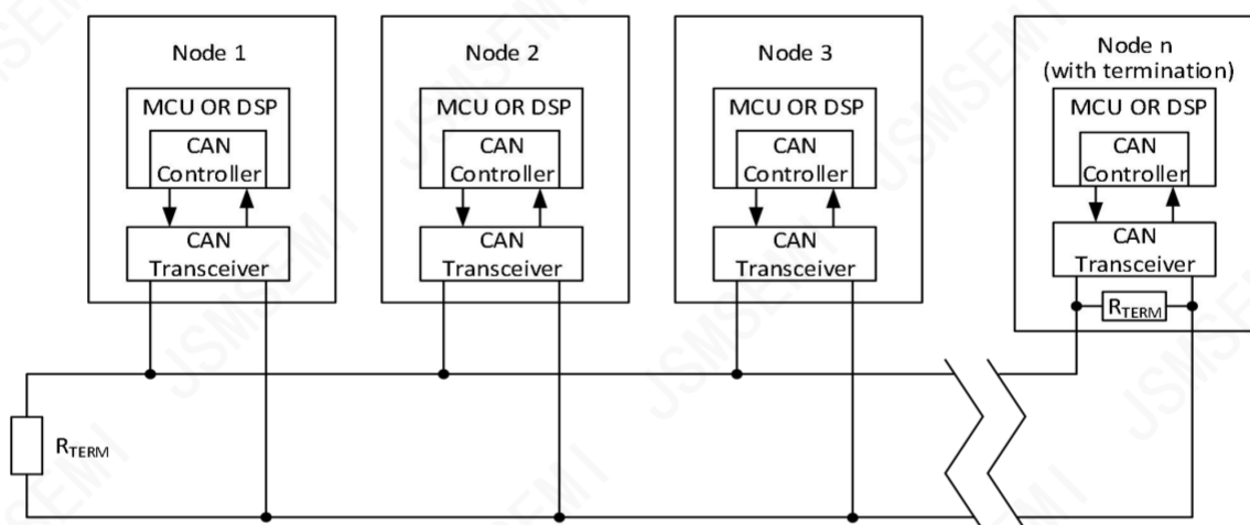
Figure 7-1. Typical CAN Bus Application
