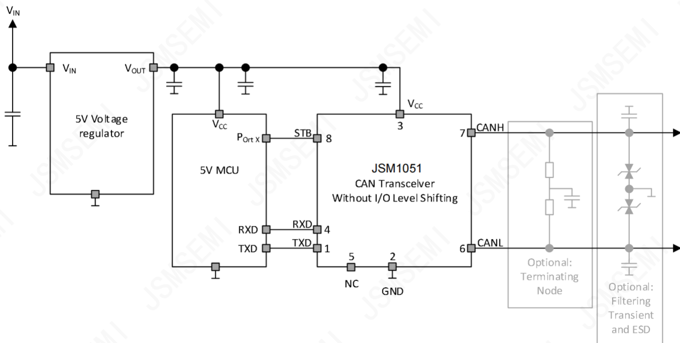
Figure 7-3. Typical CAN Bus Application Using 5V CAN Controller
