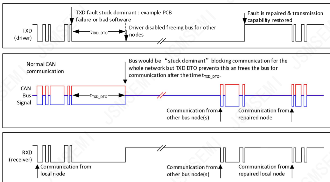
Figure6-1. Example Timing Diagram for TXD DTO
