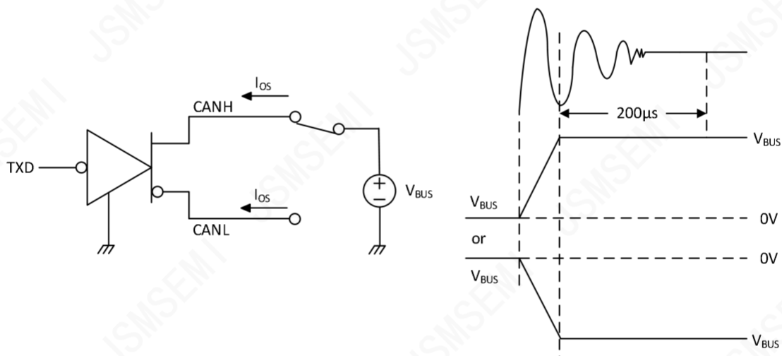
Figure5-7. Driver Short Circuit Current Test and Measurement
