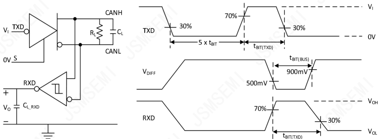
Figure5-5. CAN FD Timing Parameter Measurement
