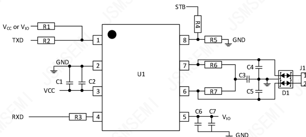
Figure 9-1. Layout Example
