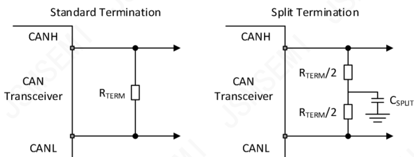
Figure 7-2. CAN Bus Termination Concepts
