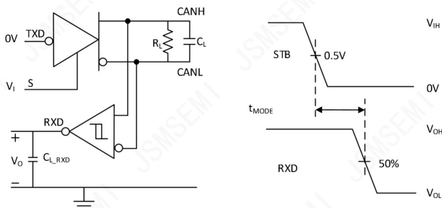
Figure5-4. T_{PROP(LOOP)} Test Circuit and Measurement
