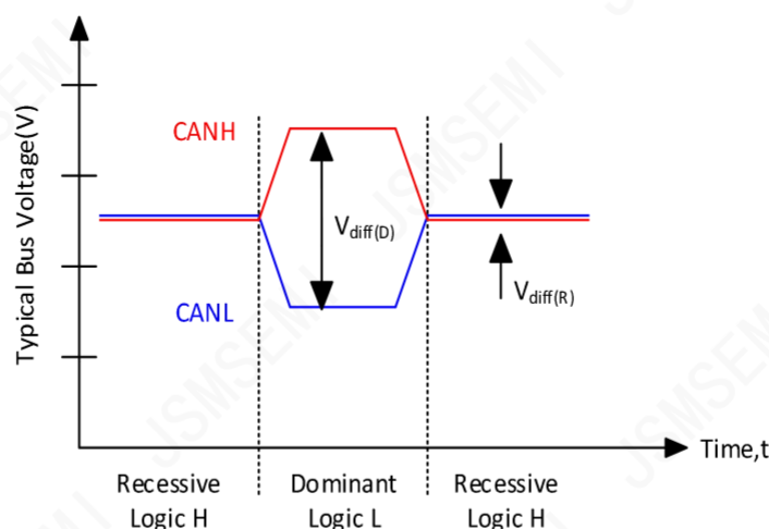
Figure 6-2. Bus States (Physical Bit Representation)
