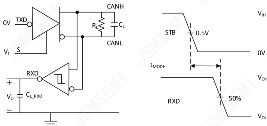
Figure5-3. t_{MODE} Test Circuit and Measurement
