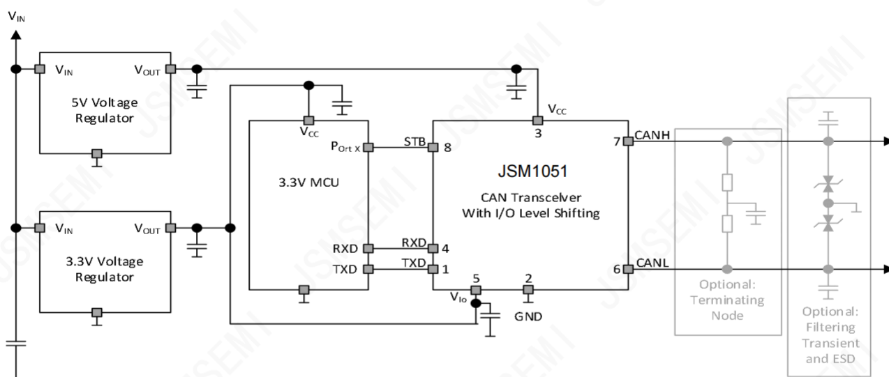
Figure 7-4. Typical CAN Bus Application Using 3.3V CAN Controller
