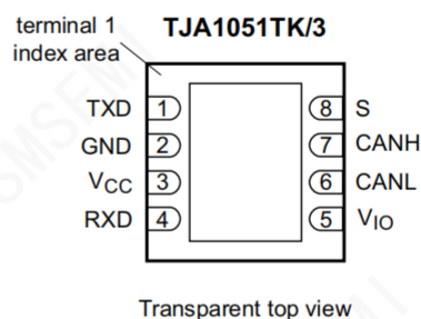
d. TJA1051TK/3: DFN-8
