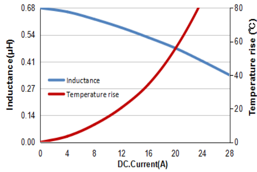
FSA0650-R68MT
