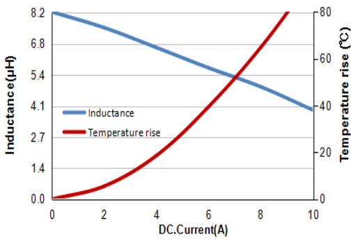
FSA0650-8R2MT
