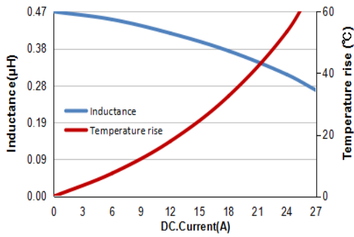
FSA0650-R47MT
