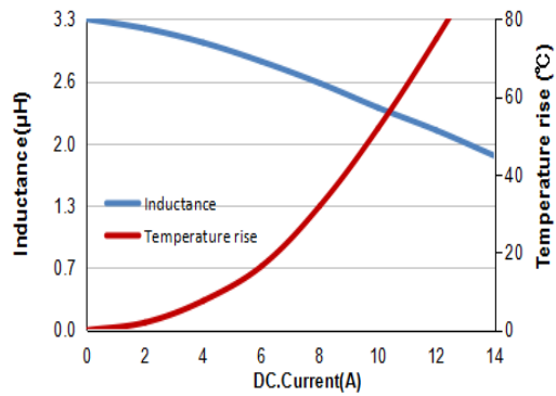
FSA0650-3R3MT
