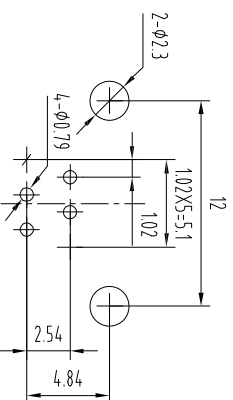
PC Board Layout Component Side Shown
