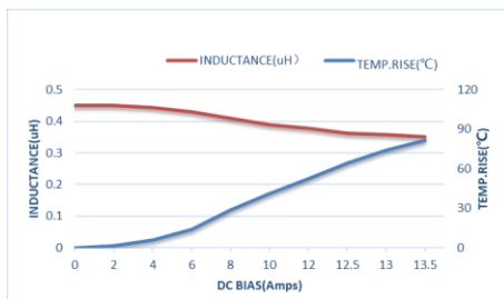
ZEP1M322520TR47MLF
