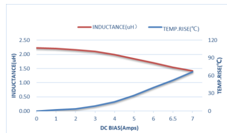
ZEP1M322520T2R2MLF
