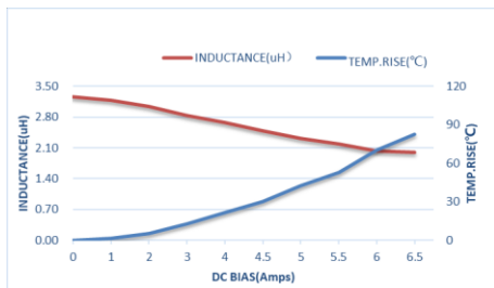
ZEP1M322520T3R3MLF
