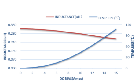
ZEP1M322520TR33MLF
