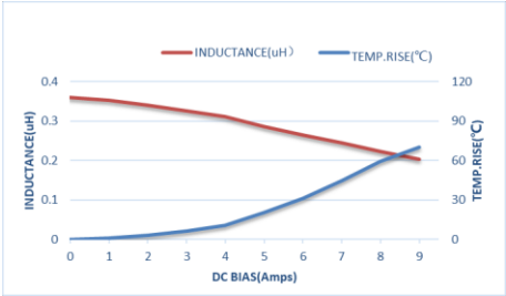
ZEPIM201608S-R33M
