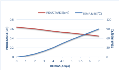
ZEPIM201608S-R68M
