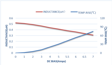
ZEPIM201608S-R47M
