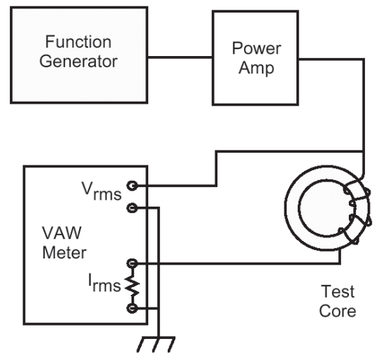
Test set up for measuring power loss.
