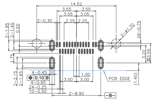
RECOMMENDED PCB PAD LAYOUT TOLERANCE:0.05mm
