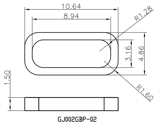
防水圈尺寸图 DIMENSION DIAGRAM OF WATERPROOF RING
