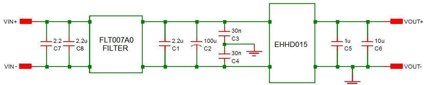
Figure 29. EMC Considerations
