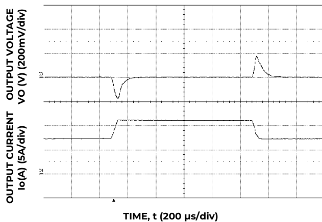
Figure 3. Transient Response to 0.1A/μS Dynamic Load Change from 50% to 75% to 50% of full load, V_{in}=24V , C_o>100\mu F .
