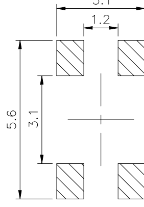
PCB. 焊接图 PCB. WELDING DRAWING
