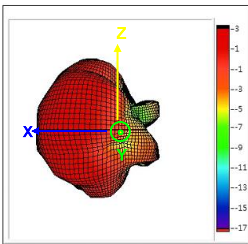
7-2. 3D Gain Pattern @ 5350 MHz (unit: dBi)
