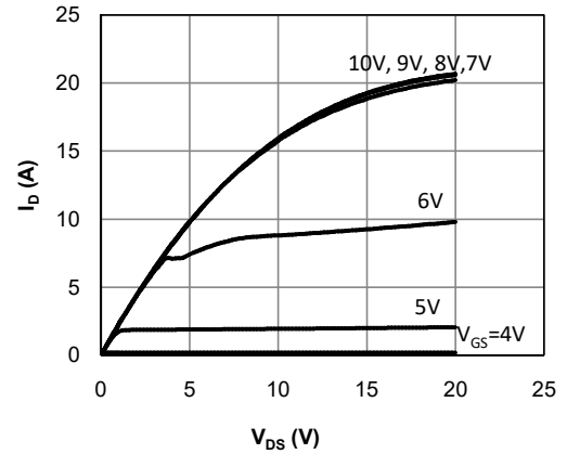
Fig 2. Output Characteristics ( T_J=150^\circ\text{C} )
