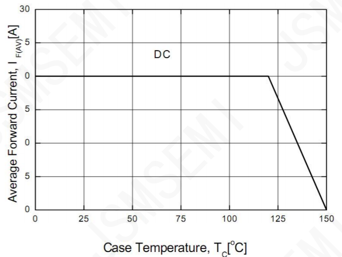
Figure 4. Power Derating
