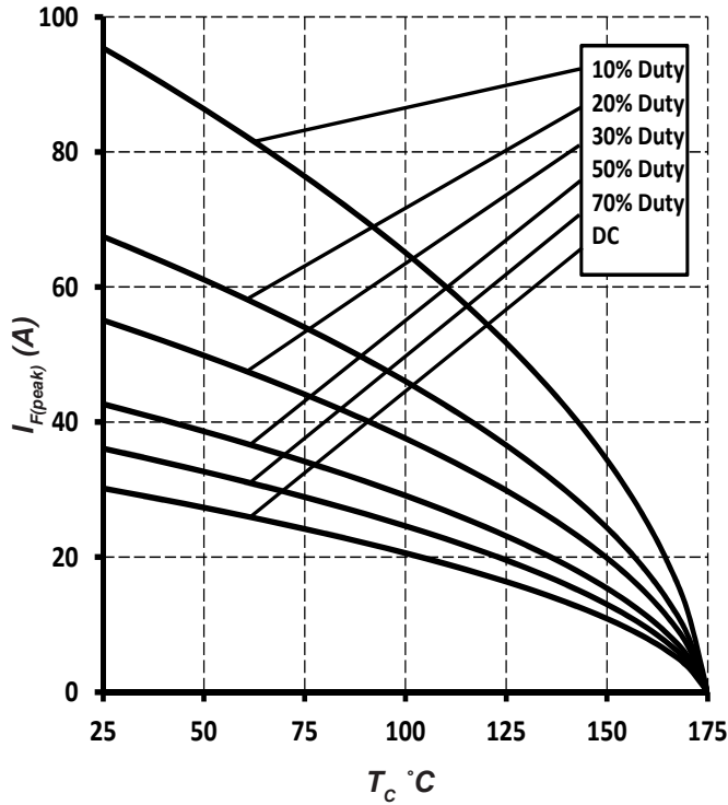
Figure 3. Current Derating
