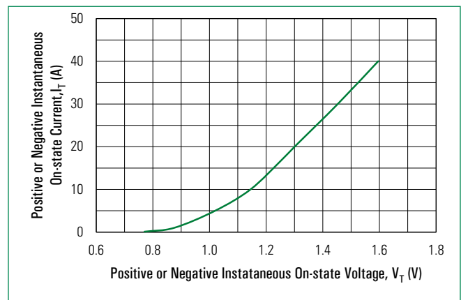
Figure 6: On-State Current vs. On-State Voltage (Typical)
