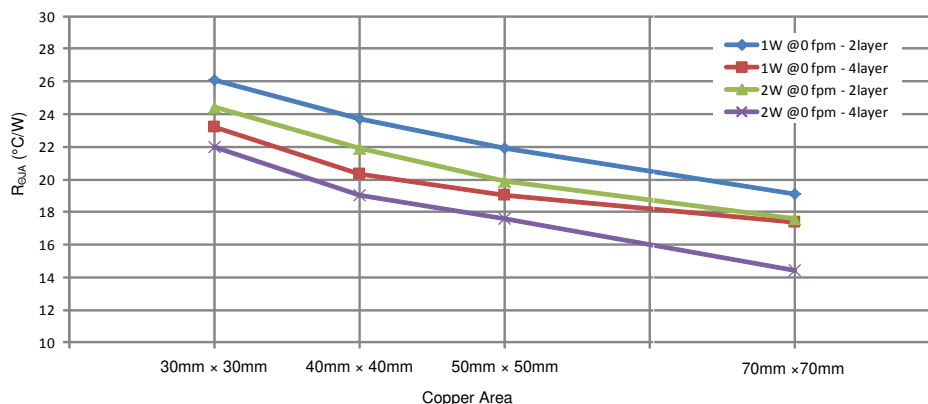
图 86. Measured R_{\theta JA} vs PCB Copper Area on a 2-Layer Board and a 4-Layer Board
