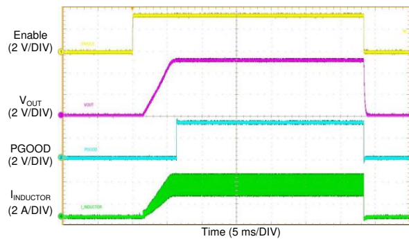
图 65. LM76003 Start-up Waveform
