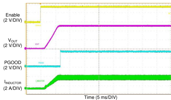
图 67. Start-up Waveform
