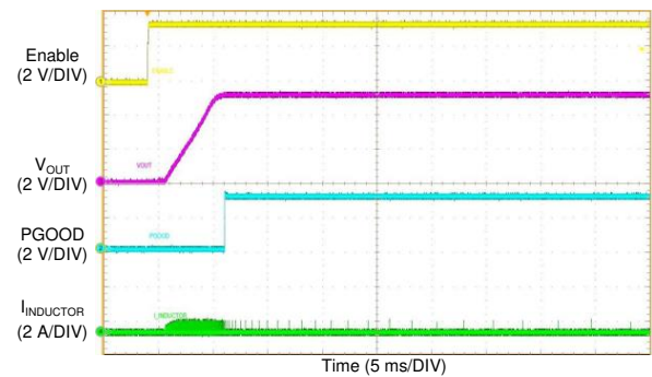
图 66. LM76003 Start-up Waveform
