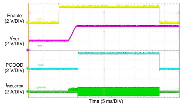
图 68. LM76002 Start-up Waveform
