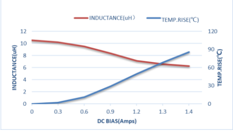
ZETC201608S-100MT-LF
