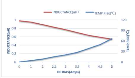
ZETC201608S-1R0MT-LF
