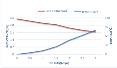
ZETC201608S-3R3MT-LF
