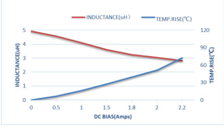
ZETC201608S-4R7MT-LF
