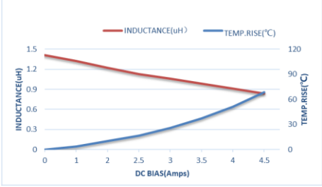
ZETC201608S-1R5MT-LF
