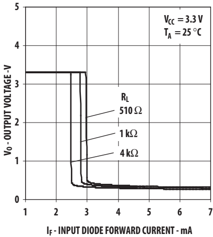
Figure 2: Input-Output Characteristics
